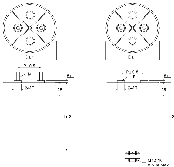
Clamp mounting
